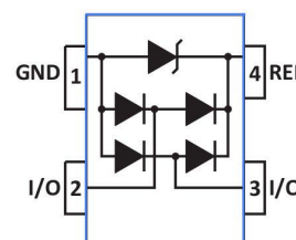
Schematic and PIN Configuration
