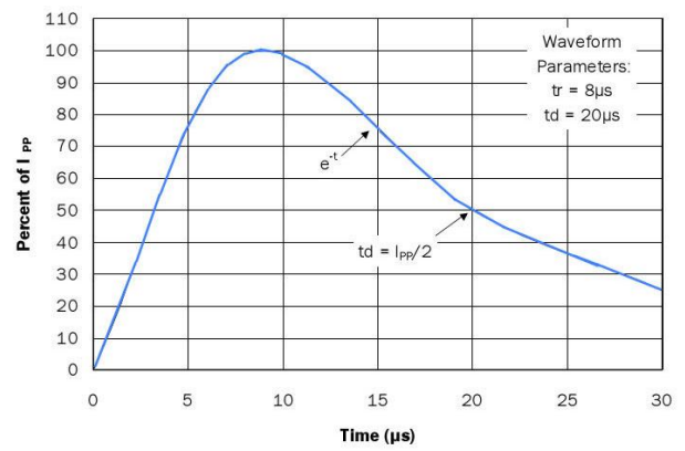
Figure 2- Pulse Waveform
