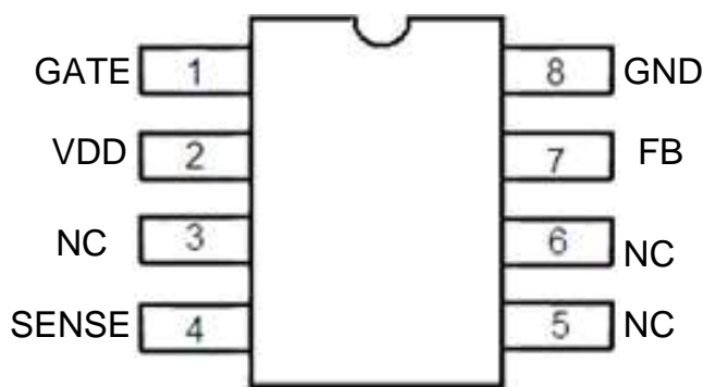
DIP8
