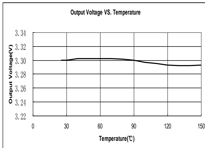
ME6118A33B3G ( V_{IN}=V_{OUT}+1.2V , I_{OUT}=10mA )
