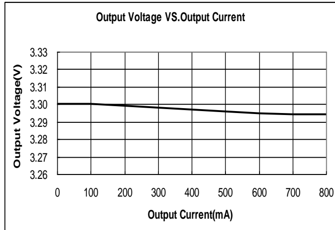
ME6118A33B3G ( V_{IN}=V_{OUT}+1.2V )
