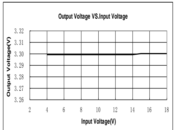
ME6118A33B3G
