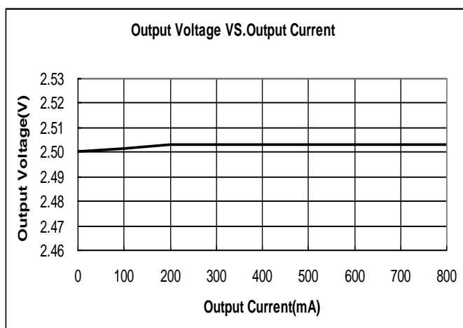
ME6118A25B3G ( V_{IN}=V_{OUT}+1.2V )
