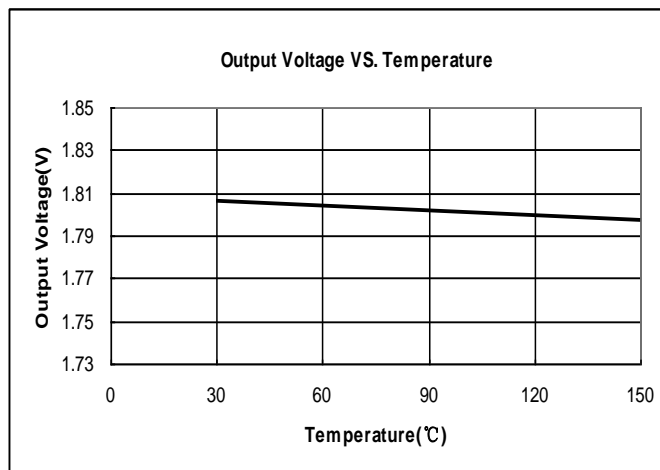
ME6118A18B3G ( V_{IN}=V_{OUT}+1.2V , I_{OUT}=10mA )
