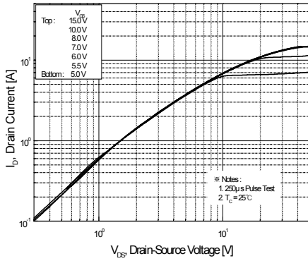
Figure 1. On-Region Characteristics
