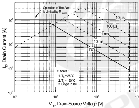
Figure 9-2. Maximum Safe Operating Area for WGF7N65
