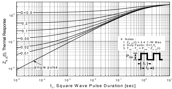
Figure 11-2. Transient Thermal Response Curve for WGF7N65
