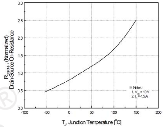
Figure 8. On-Resistance Variation
