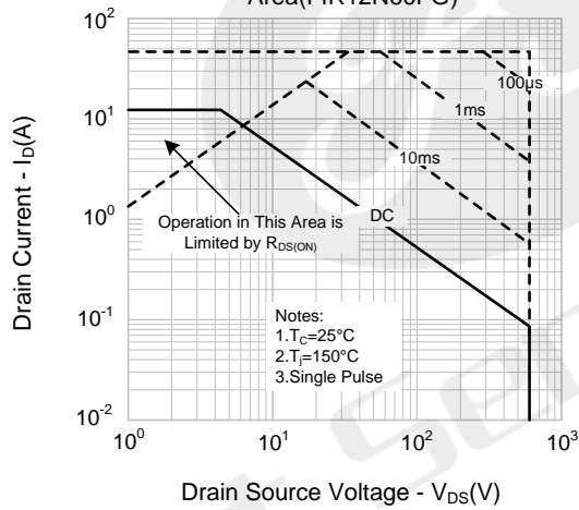
Figure 9-2. Max. Safe Operating Area(FIR12N60FG)
