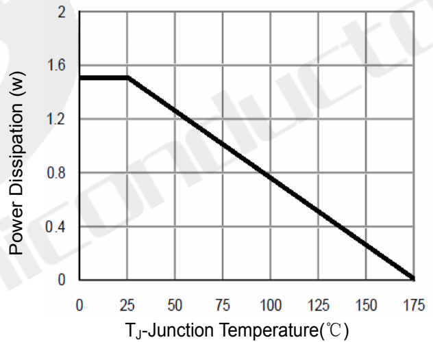
Figure 10 Power De-rating
