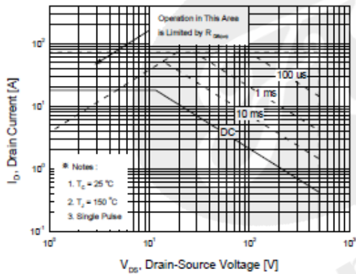
Figure 9-1. Maximum Safe Operating Area for FQP18N50V2
