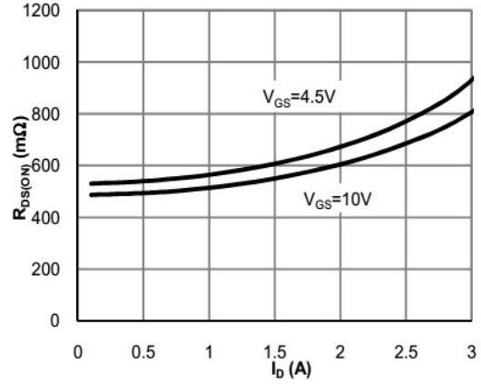
Figure 2. On-Resistance Characteristics
