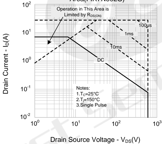
Figure 9. Max. Safe Operating Area(FIR7N60LG)
