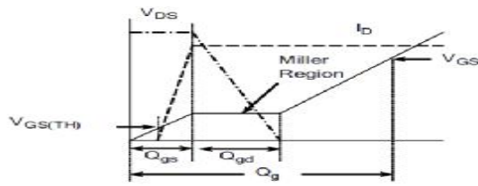
Figure 18. Gate Charge Waveform
