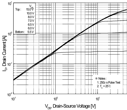
Figure 1. On-Region Characteristics
