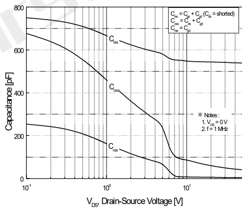
Figure 5. Capacitance Characteristics
